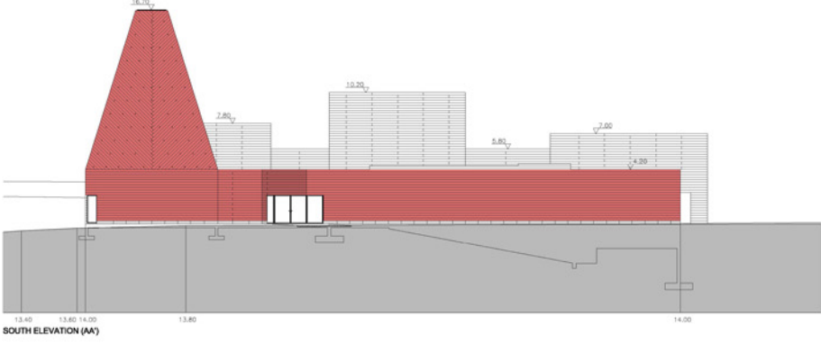
SOUTH ELEVATION (AV)
