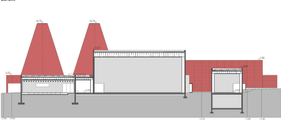
SECTION 6
