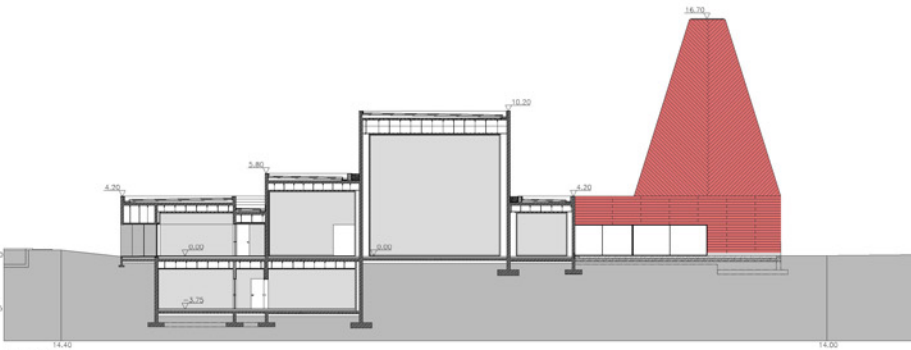
SECTION 3
