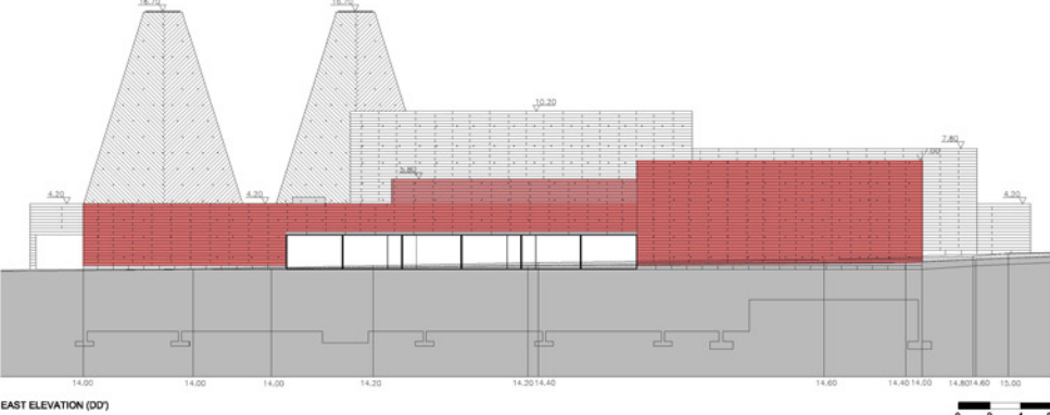
EAST ELEVATION (DD')
