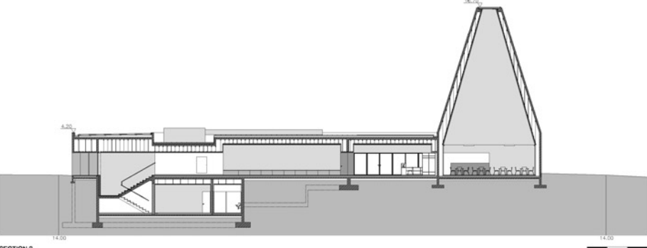
SECTION 2
