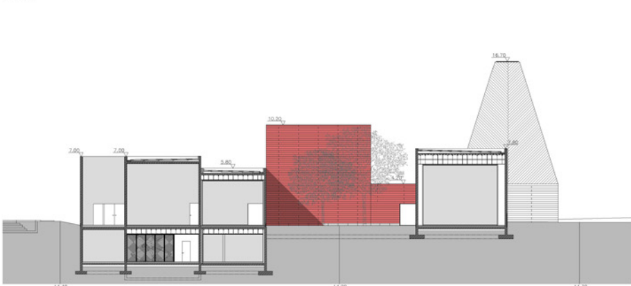
SECTION 5
