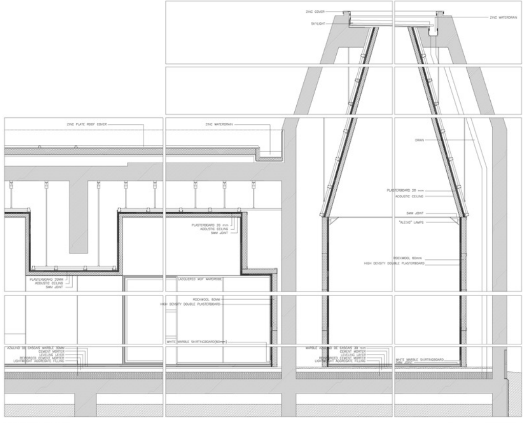
CONSTRUCTIVE SECTION 2
