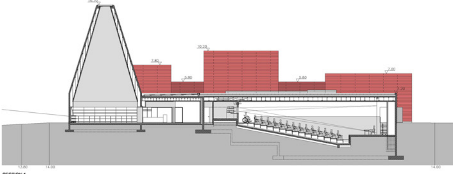
SECTION 1
