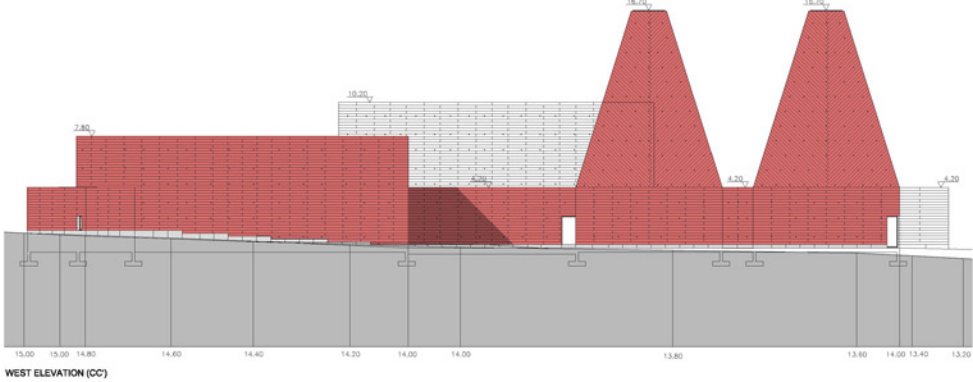
WEST ELEVATION (CC')
